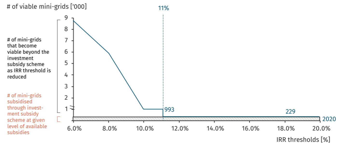
Figure 48. Simulation of number of viable mini-grids for different levels of IRR threshold in 2020. Assumes current investment subsidy scheme (DRD covers 60% of capital costs, community contribution covers 20% of capital costs and developer covers remaining 20% of capital costs) and 18.6 million USD subsidies budget;
